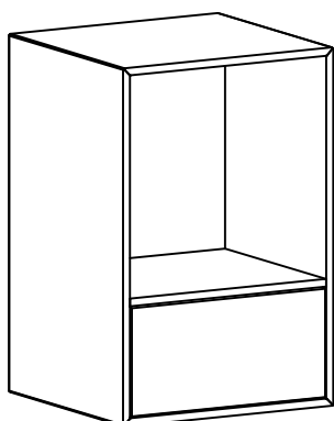
Template no. 1 Place against the bottom Mark A + Template no. 3 Place against the bottom Mark J
